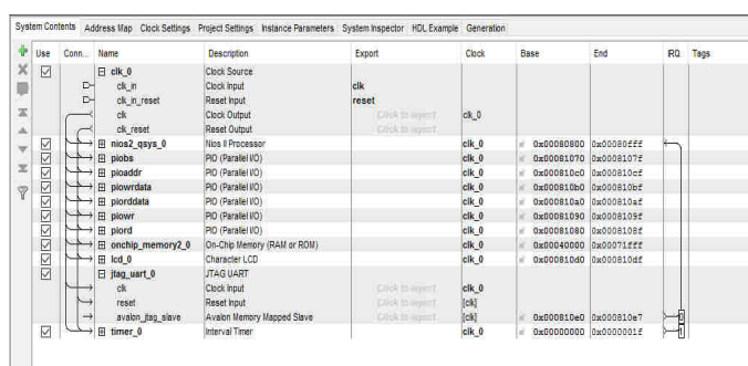
Fig.3: Qsys Structure of Proposed Work
